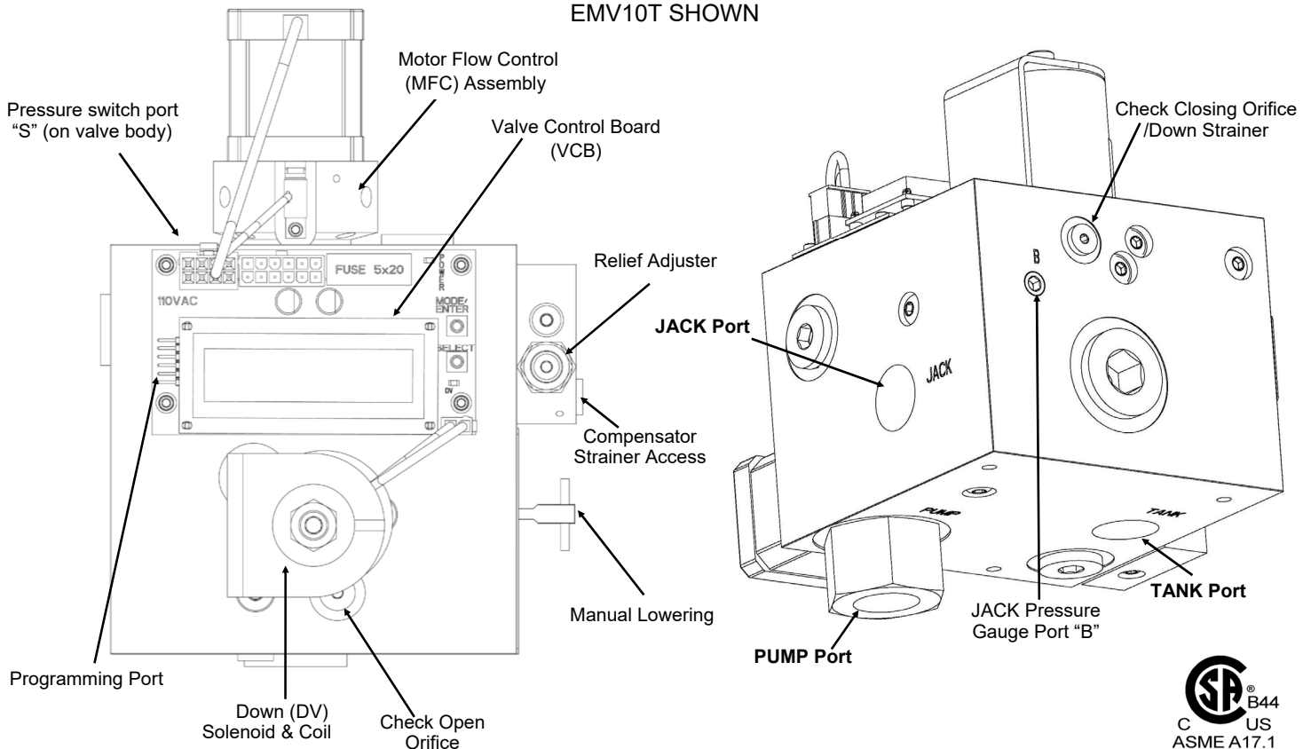
EMV10T SHOWN
